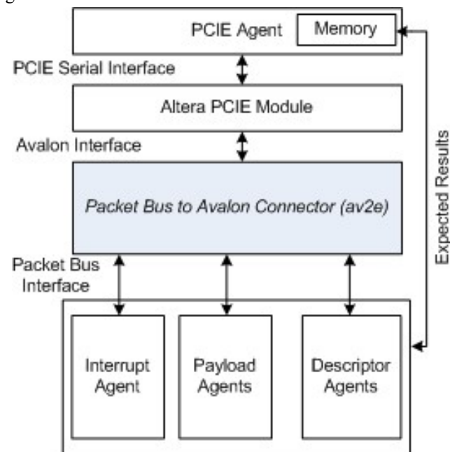
Fig. 3. Structure of av2e module test system.
